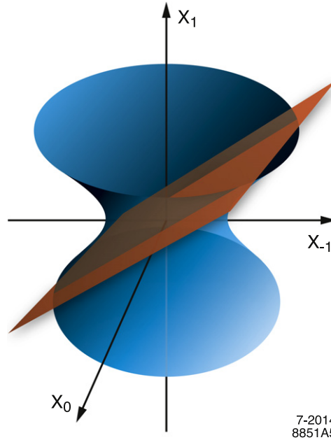
Fig. A.1. The space AdS 2 embedded as the hyperboloid X_{-1}^2 + X_0^2 - X_1^2 = R^2 into a three dimensional space and the plane X_1 - X_{-1} = 0 .
